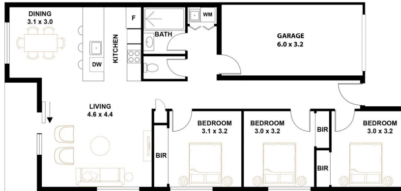
FLOOR PLAN
