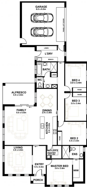
FLOOR PLAN
