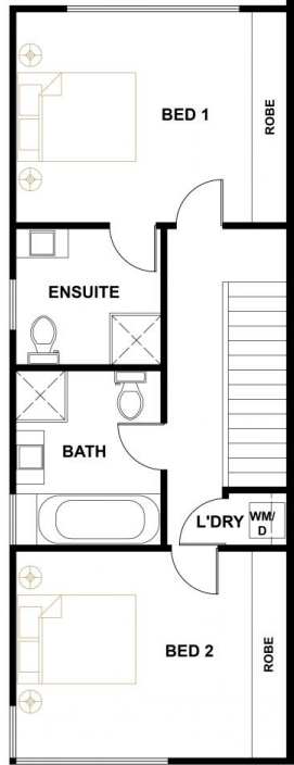
FIRST LEVEL
