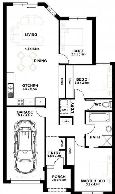
FLOOR PLAN
